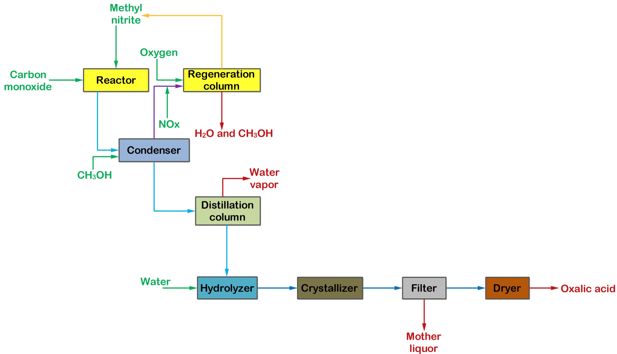
Figure: Manufacture of Oxalic acid by Dimethyl oxalate process
